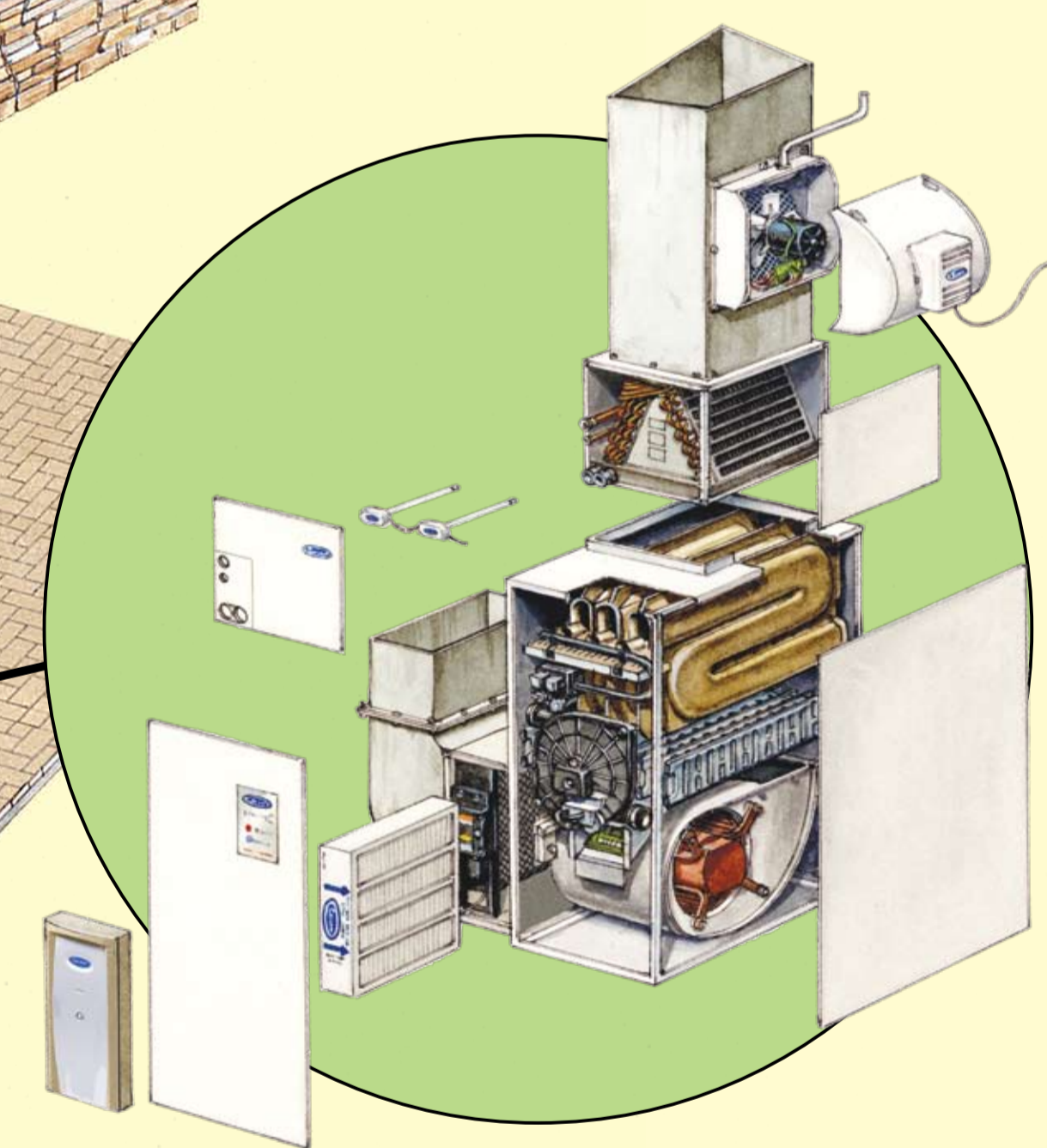
Infinity System gas furnace, air purifier, evaporator coil, UV lamps and whole house humidifier
